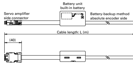
4) Encoder cable attached to battery, with connector on one end (Model no.: AL-00697960-□□)
