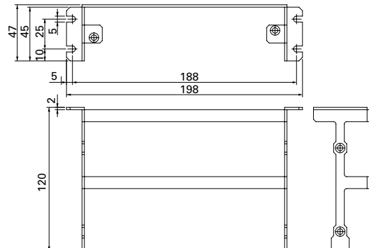
15 A (front) AL-00582788-01
