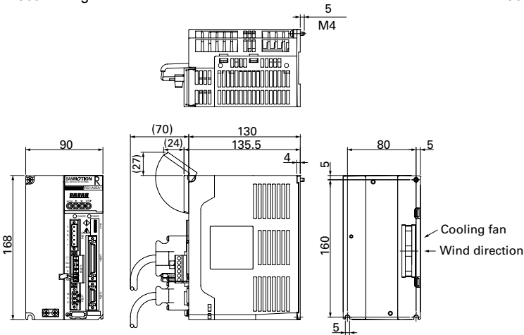
50 A Mass: 2.2 kg
