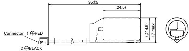
2) Replacement battery for use with battery box (Model no.: AL-00879511-01)
