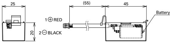
1) Battery box (Model no.: AL-00880402-01)
