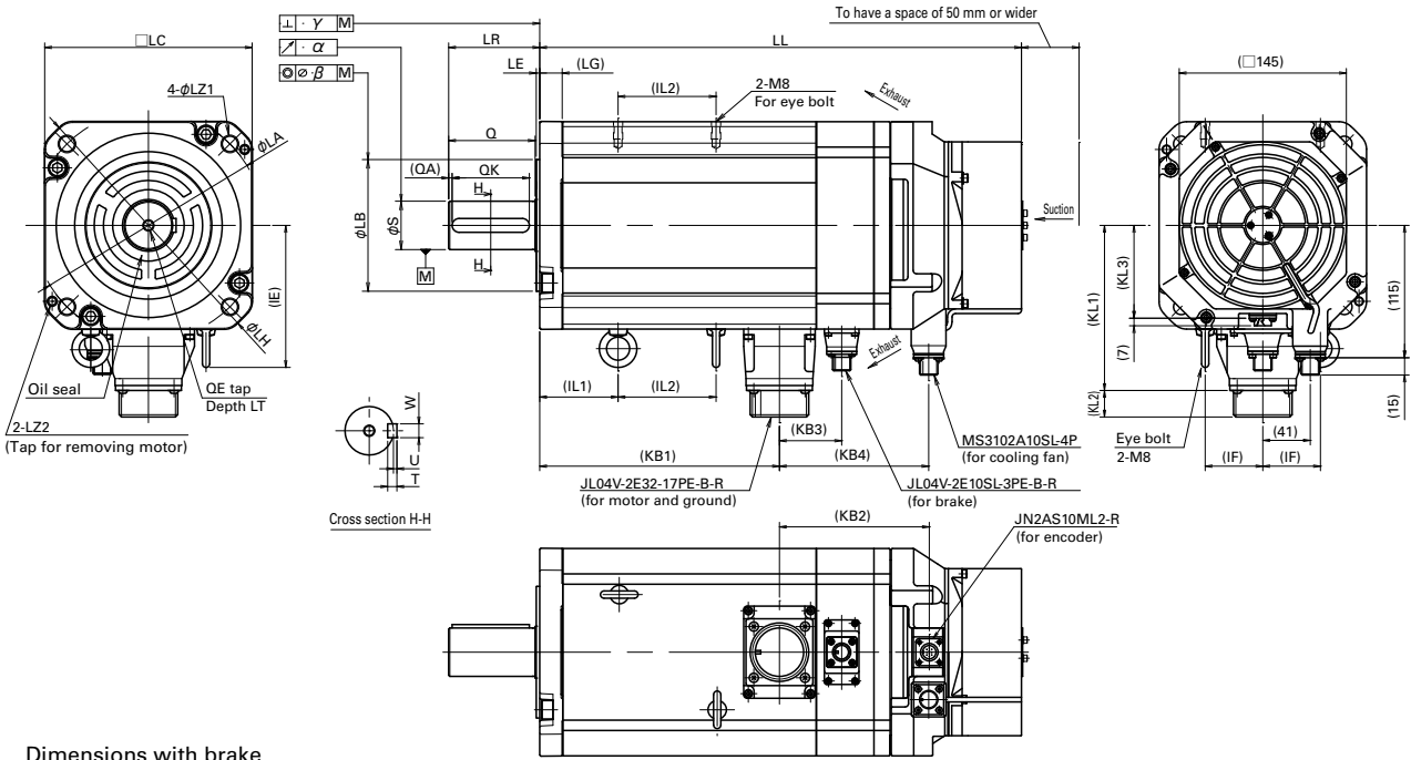
Dimensions with brake
