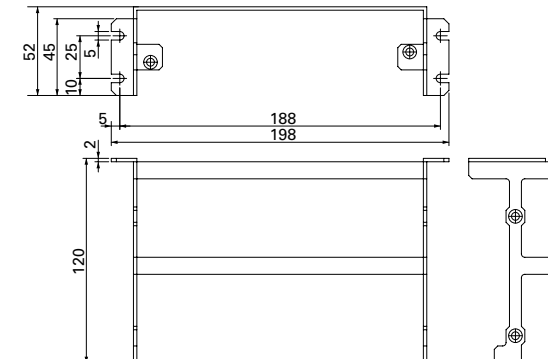
30 A (front) AL-00582789-01
