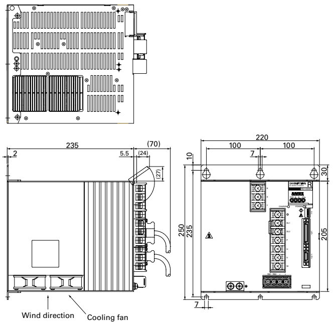
300 A Mass: 9.8 kg
