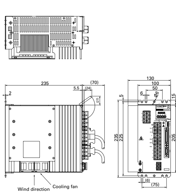
150 A Mass: 6.5 kg
