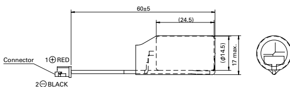
5) Replacement battery for encoder cable with battery (Model no.: AL-00697958-01)
